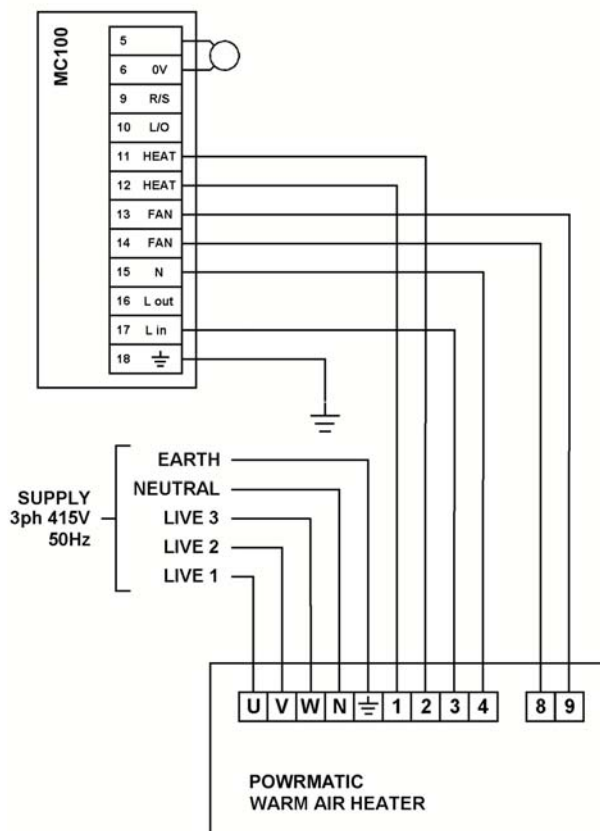
MC100 CONTROLLING 3ph CABINET HEATERS
